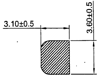
SECTION A - A SCALE 4 = 1
